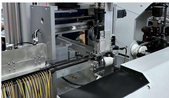
Crimp/Crimp Productivity
